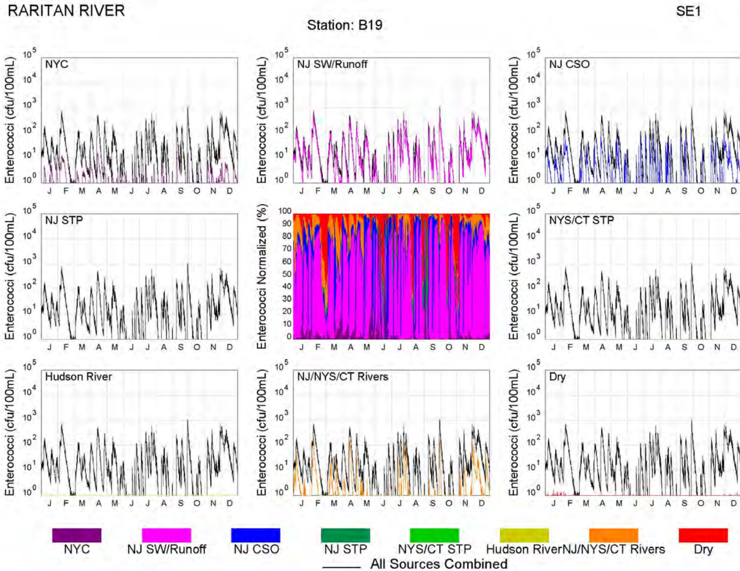
Figure 6-4. Component Analysis for Enterococci at Station B19
