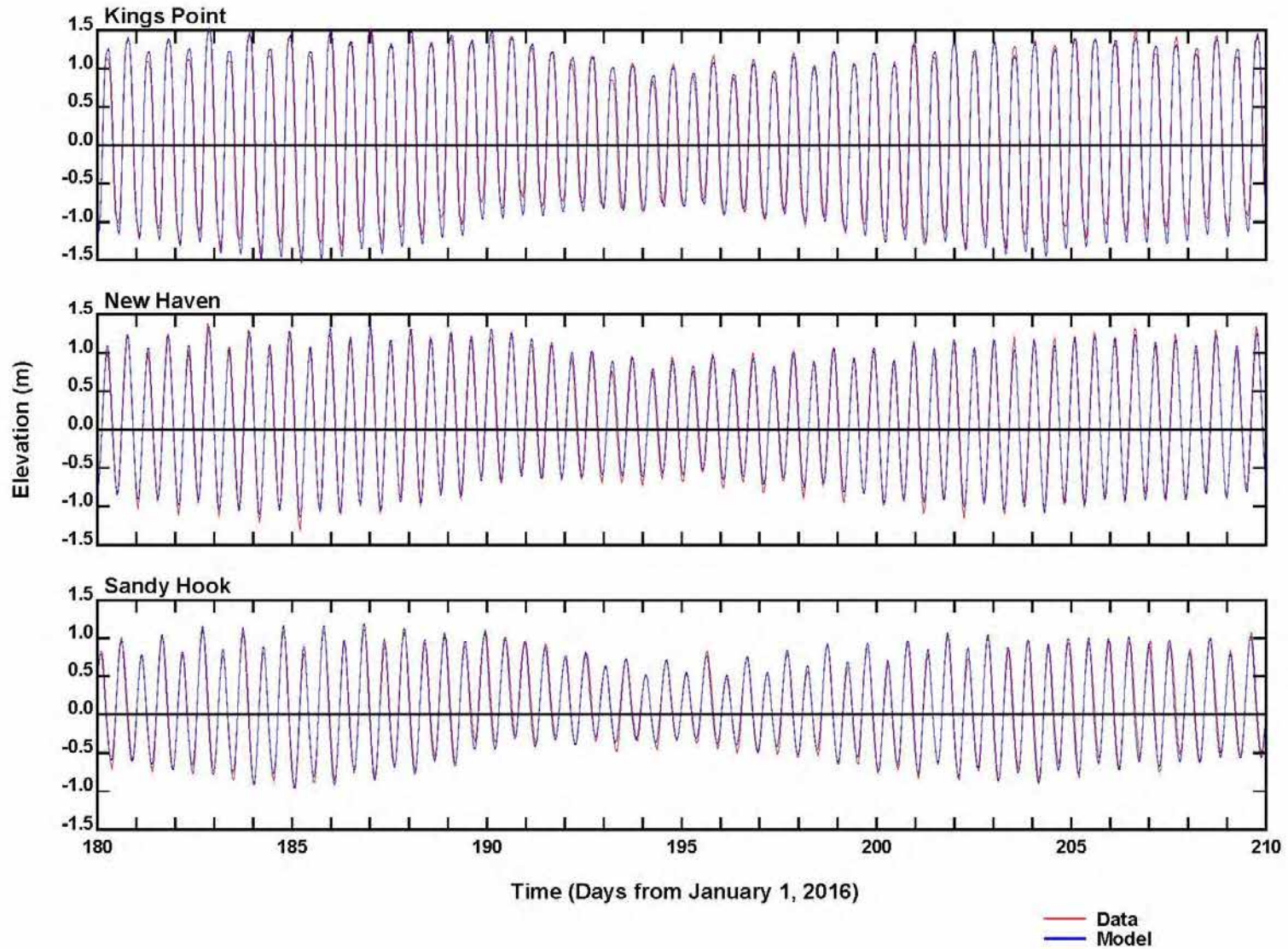
Figure 5-2. 2016 Comparison of Hourly Tidal Water Elevations (Continued)
